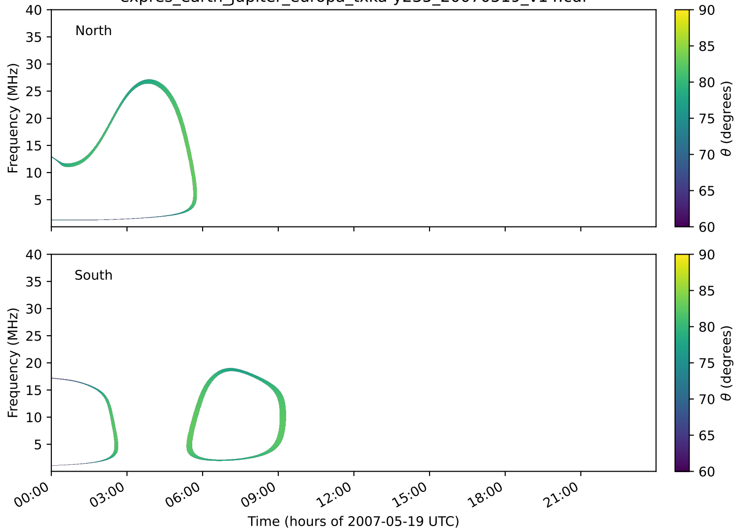
expres_earth_jupiter_europa_txka-y235_20070519_v14.cdf
