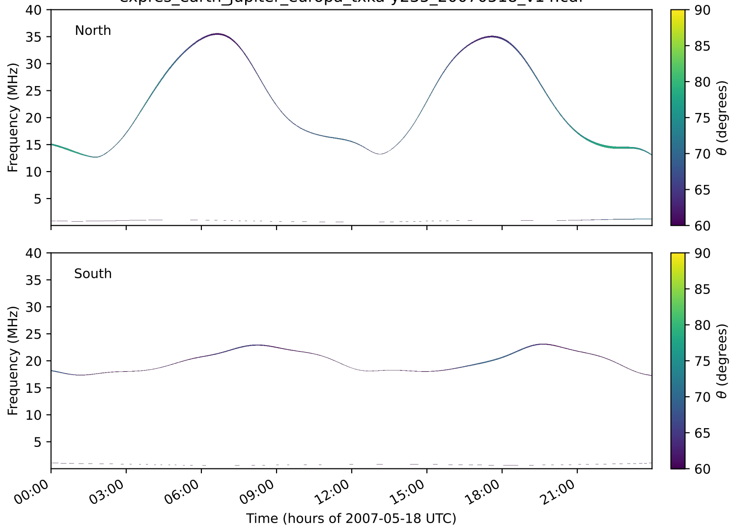
expres_earth_jupiter_europa_txka-y235_20070518_v14.cdf
