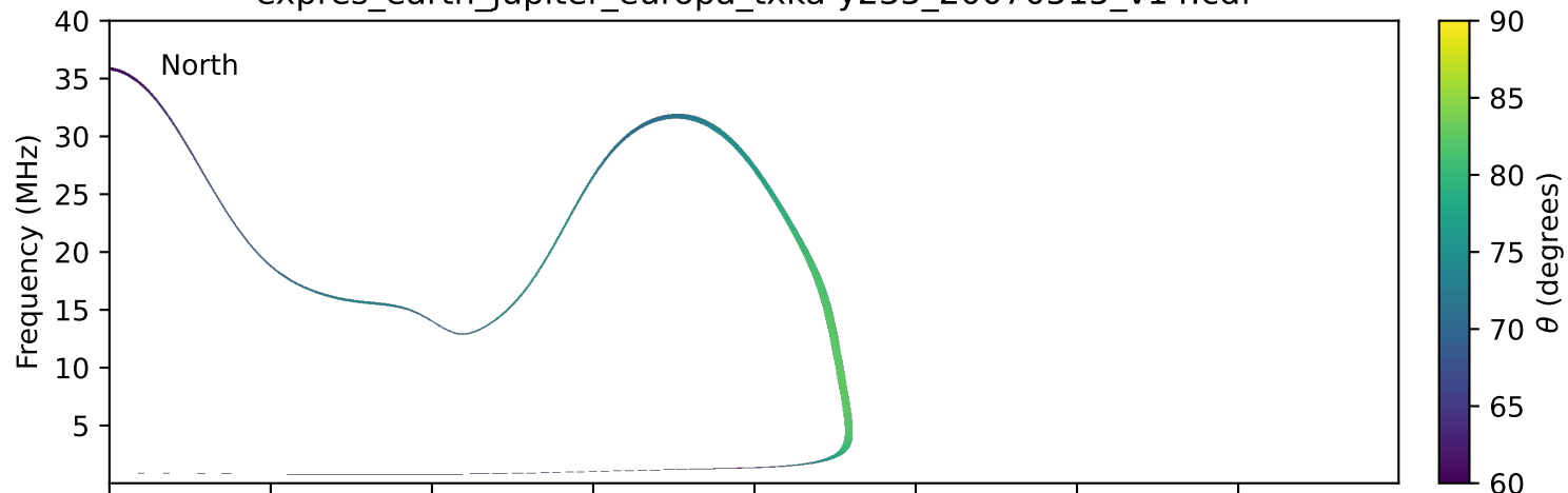
expres_earth_jupiter_europa_txka-y235_20070515_v14.cdf
