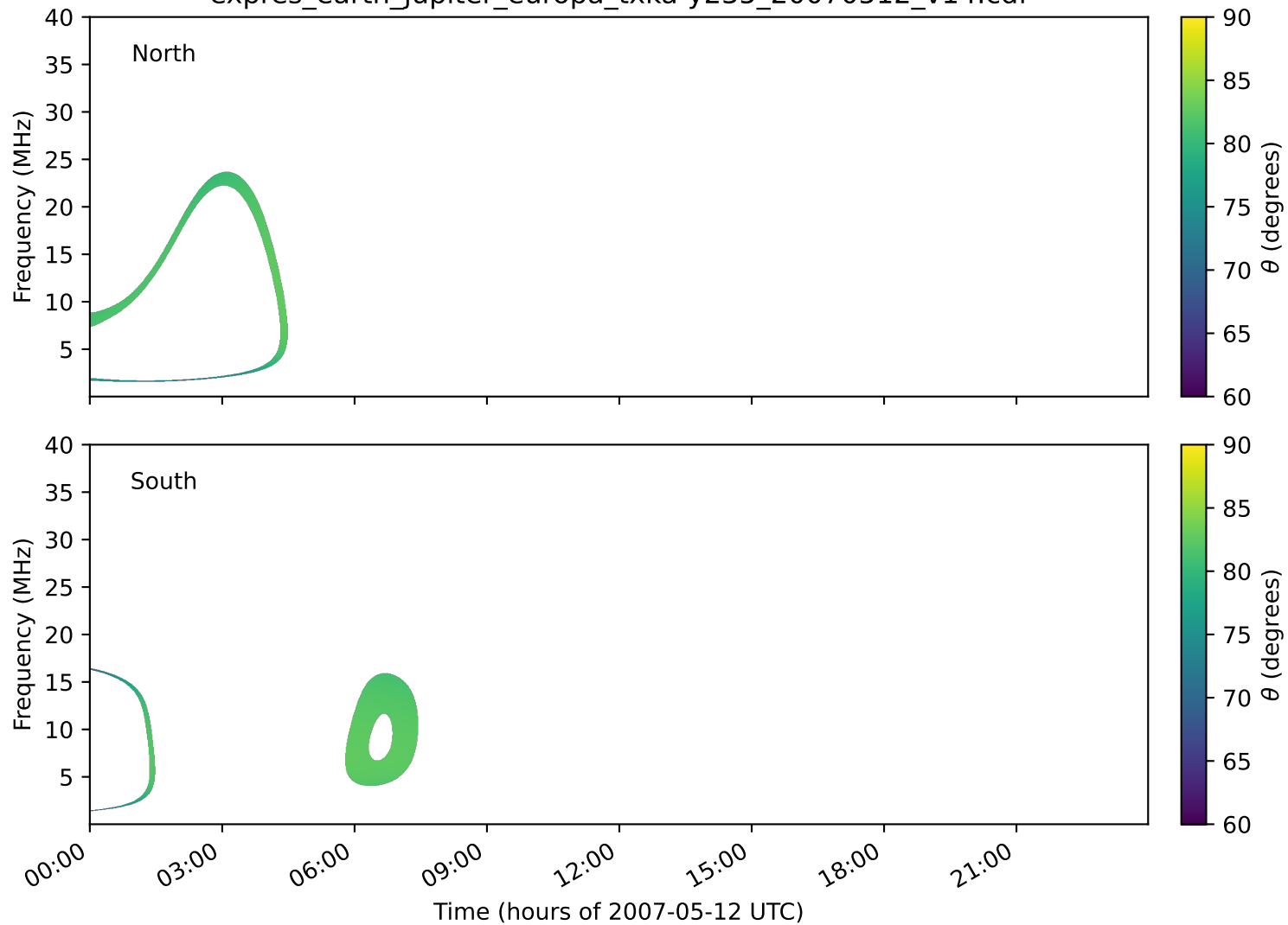
expres_earth_jupiter_europa_txka-y235_20070512_v14.cdf
