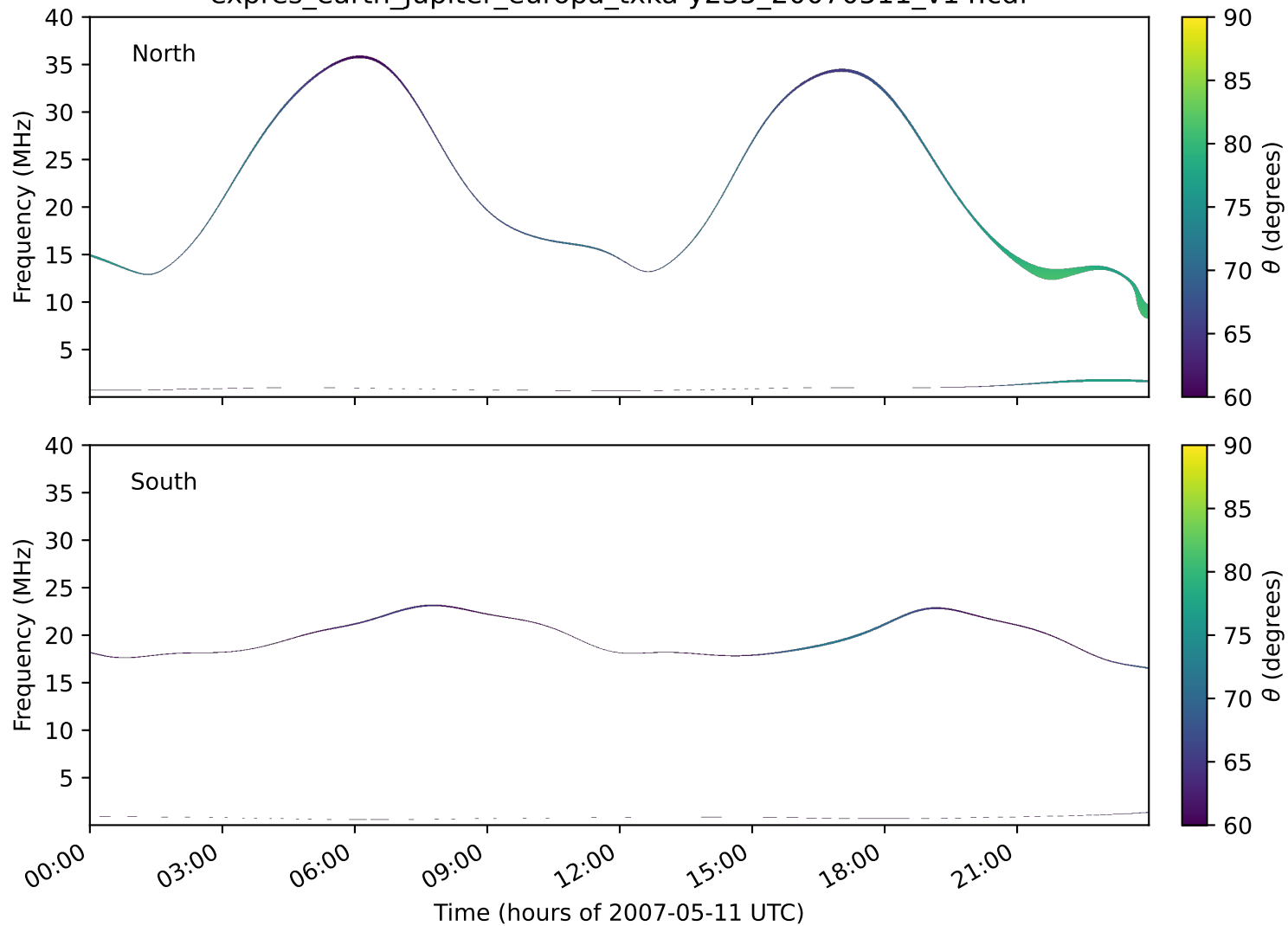
expres_earth_jupiter_europa_txka-y235_20070511_v14.cdf
