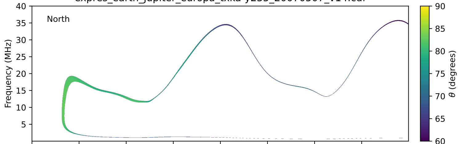
expres_earth_jupiter_europa_txka-y235_20070507_v14.cdf
