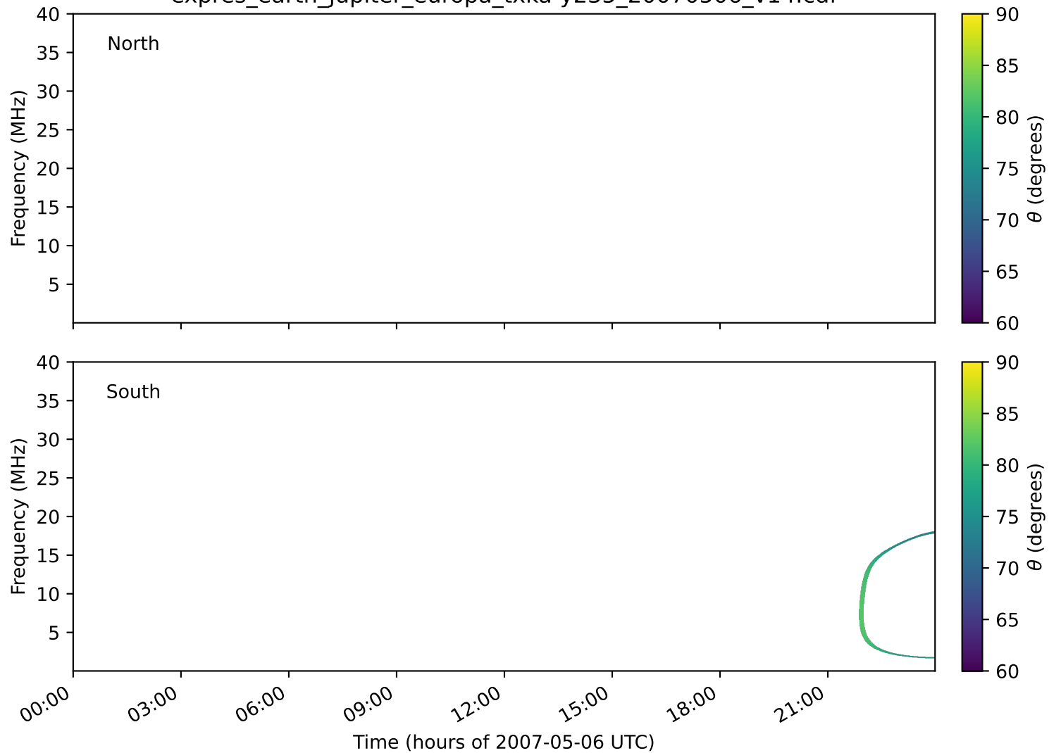
expres_earth_jupiter_europa_txka-y235_20070506_v14.cdf
