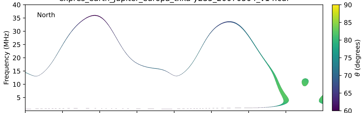
expres_earth_jupiter_europa_txka-y235_20070504_v14.cdf
