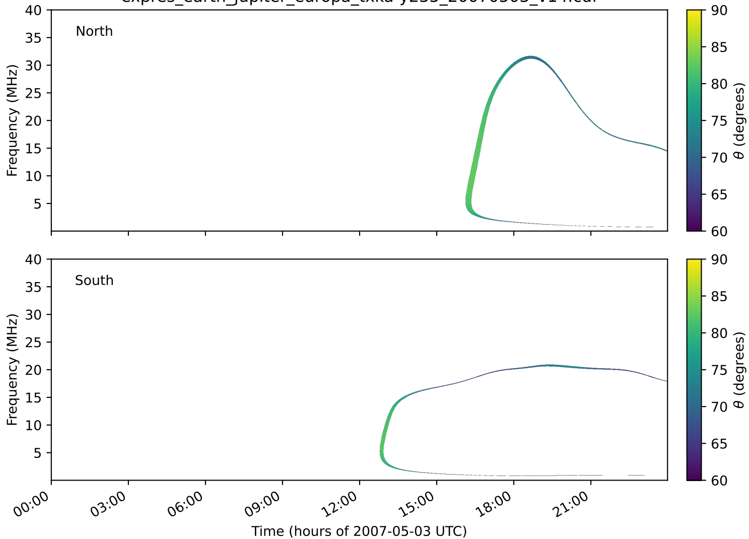
expres_earth_jupiter_europa_txka-y235_20070503_v14.cdf
