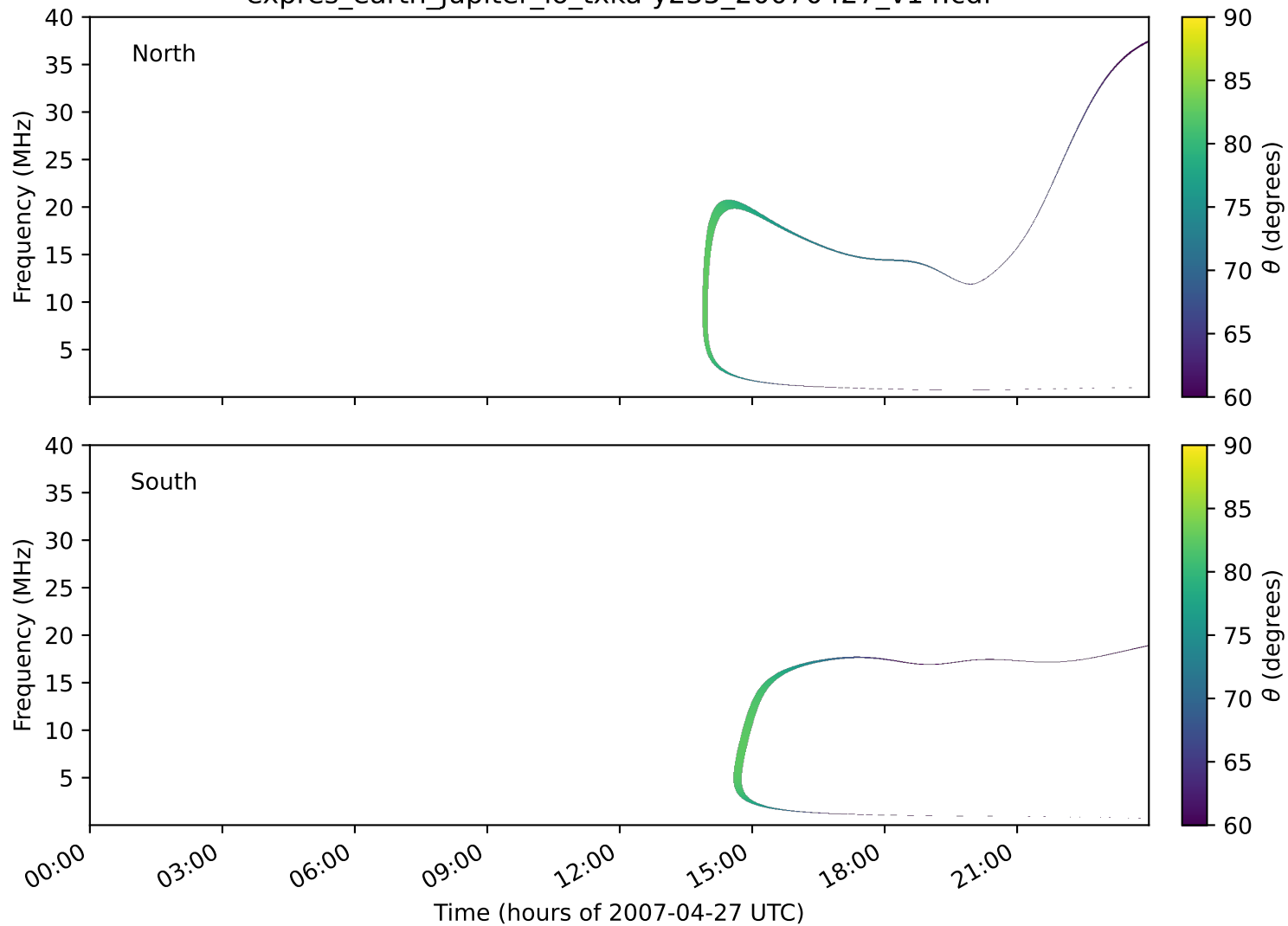
expres_earth_jupiter_io_txka-y235_20070427_v14.cdf
