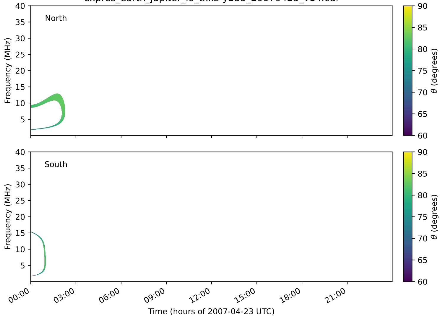
expres_earth_jupiter_io_txka-y235_20070423_v14.cdf
