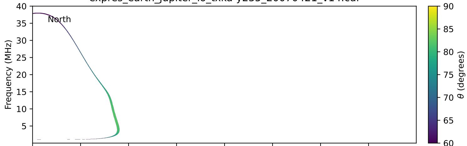
expres_earth_jupiter_io_txka-y235_20070421_v14.cdf
