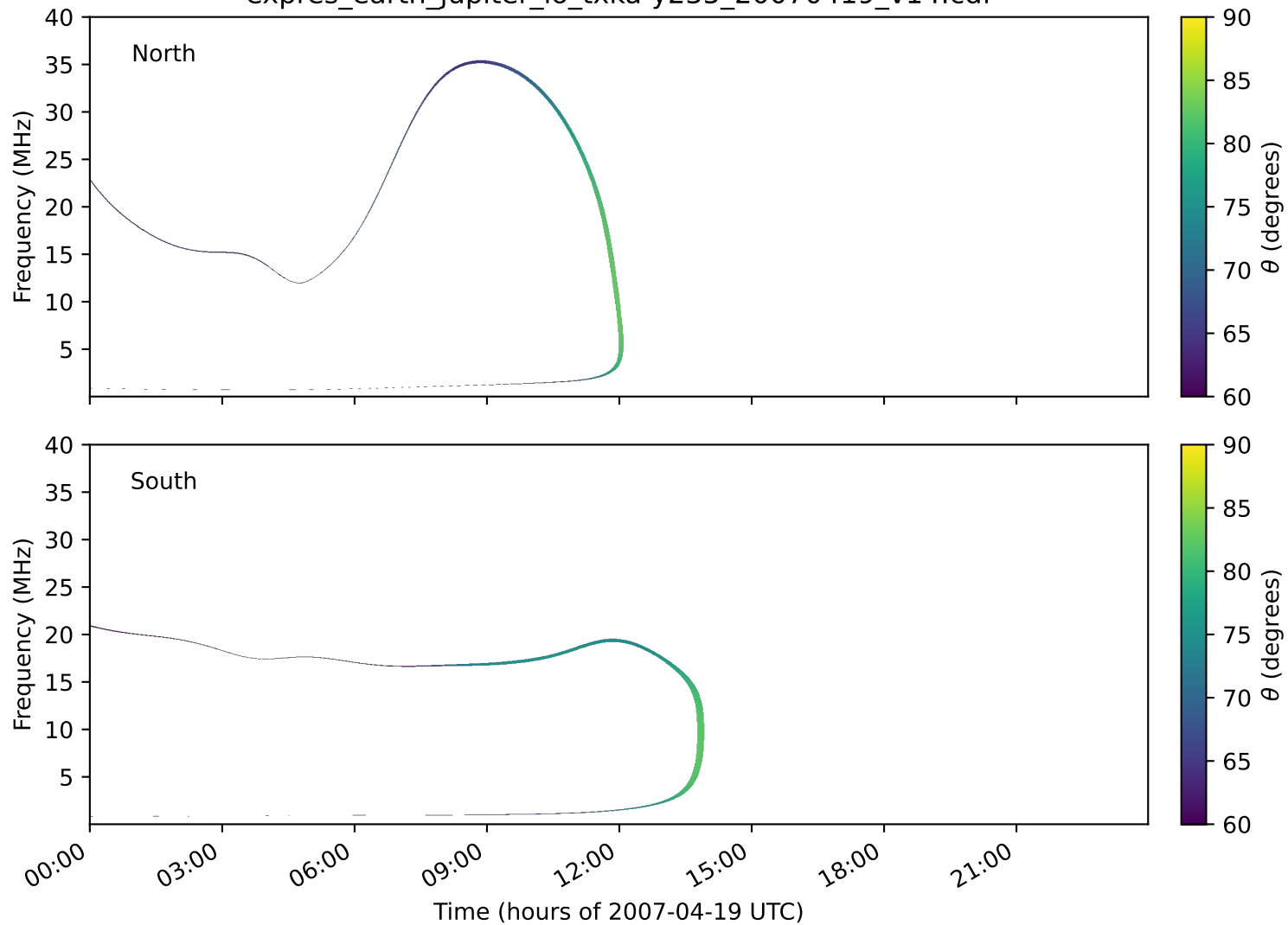
expres_earth_jupiter_io_txka-y235_20070419_v14.cdf
