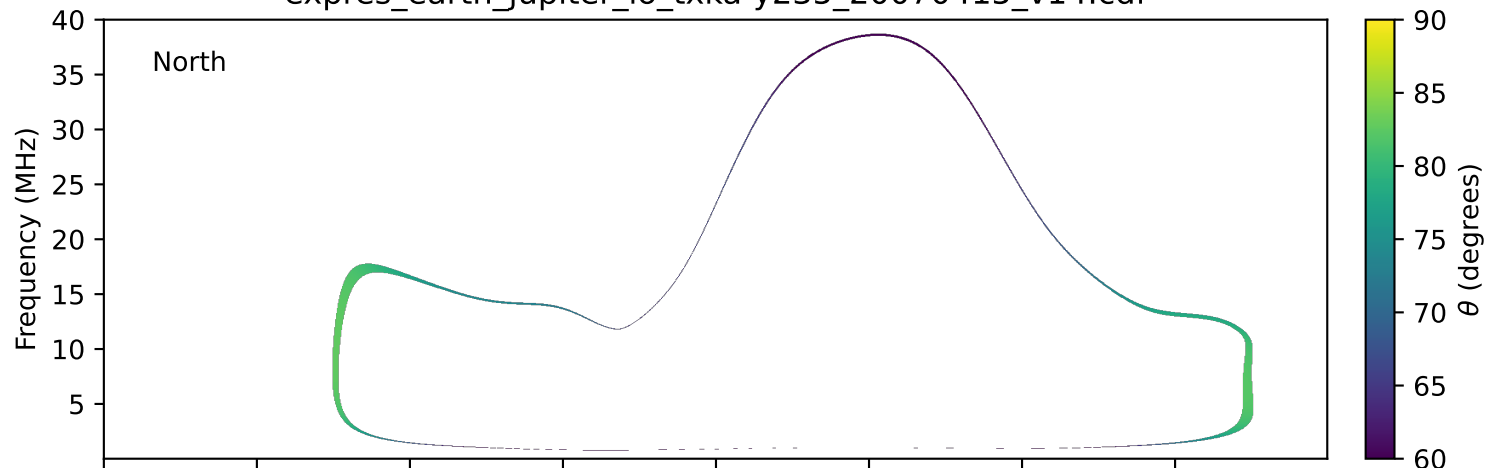
expres_earth_jupiter_io_txka-y235_20070415_v14.cdf
