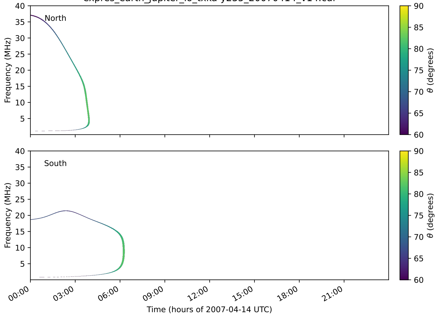
expres_earth_jupiter_io_txka-y235_20070414_v14.cdf
