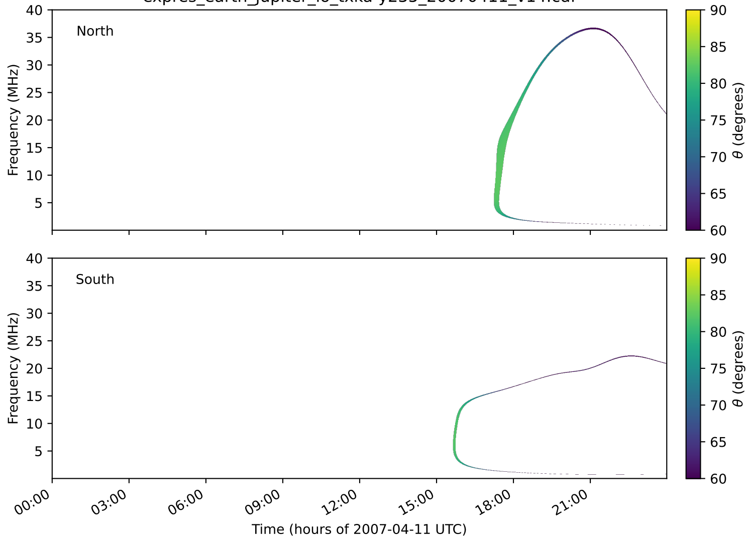
expres_earth_jupiter_io_txka-y235_20070411_v14.cdf
