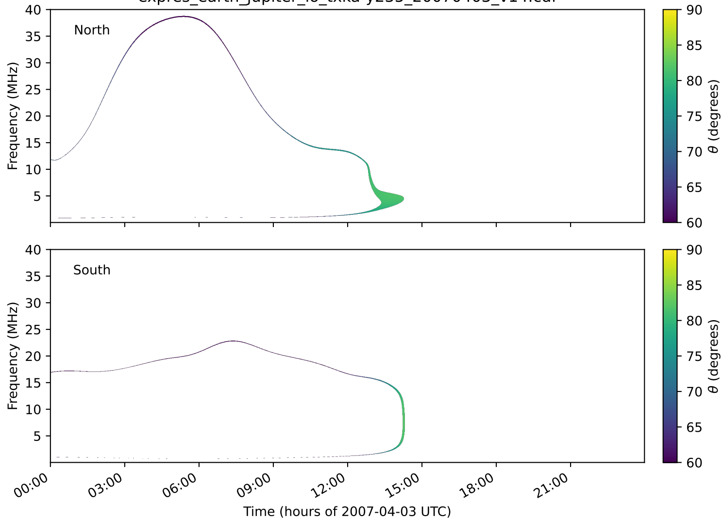
expres_earth_jupiter_io_txka-y235_20070403_v14.cdf
