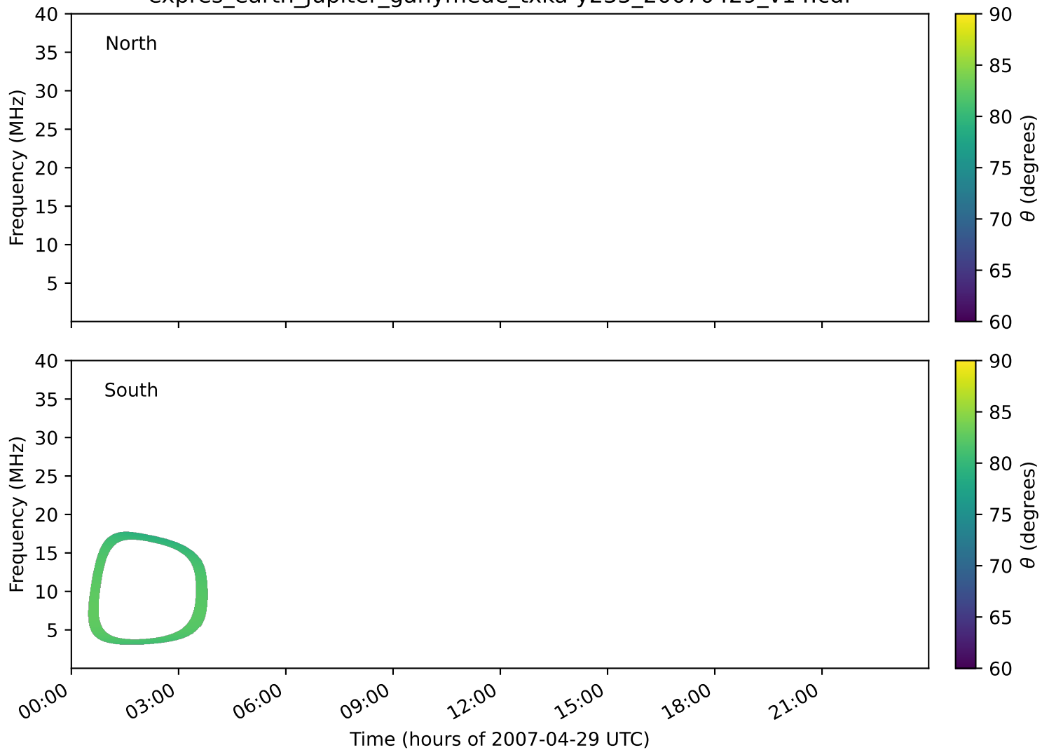
expres_earth_jupiter_ganymede_txka-y235_20070429_v14.cdf
