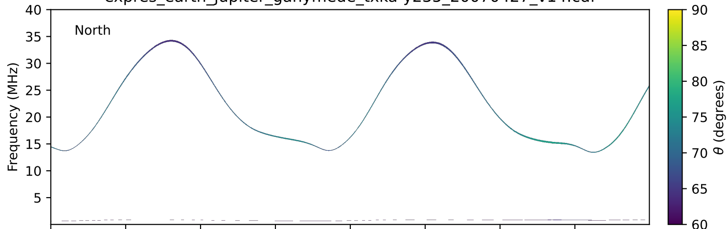
expres_earth_jupiter_ganymede_txka-y235_20070427_v14.cdf
