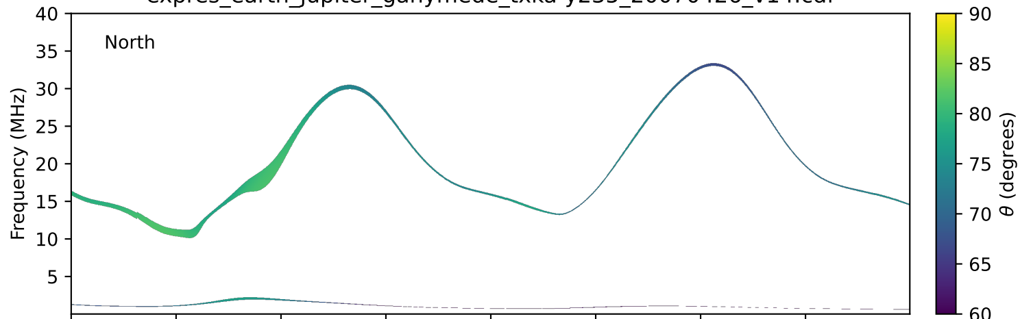
expres_earth_jupiter_ganymede_txka-y235_20070426_v14.cdf
