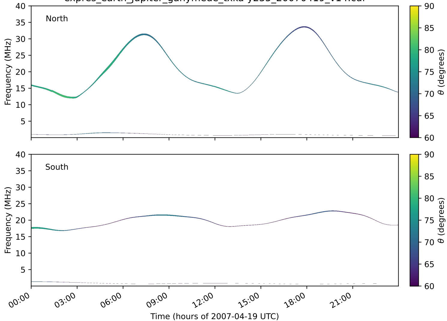
expres_earth_jupiter_ganymede_txka-y235_20070419_v14.cdf
