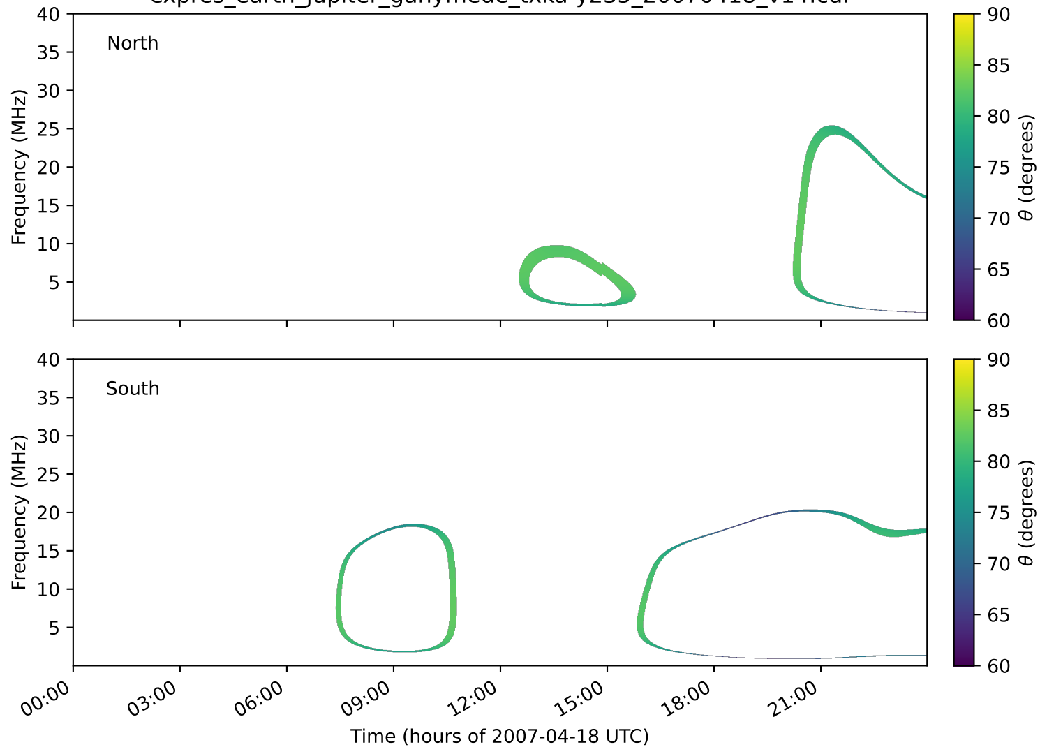
expres_earth_jupiter_ganymede_txka-y235_20070418_v14.cdf
