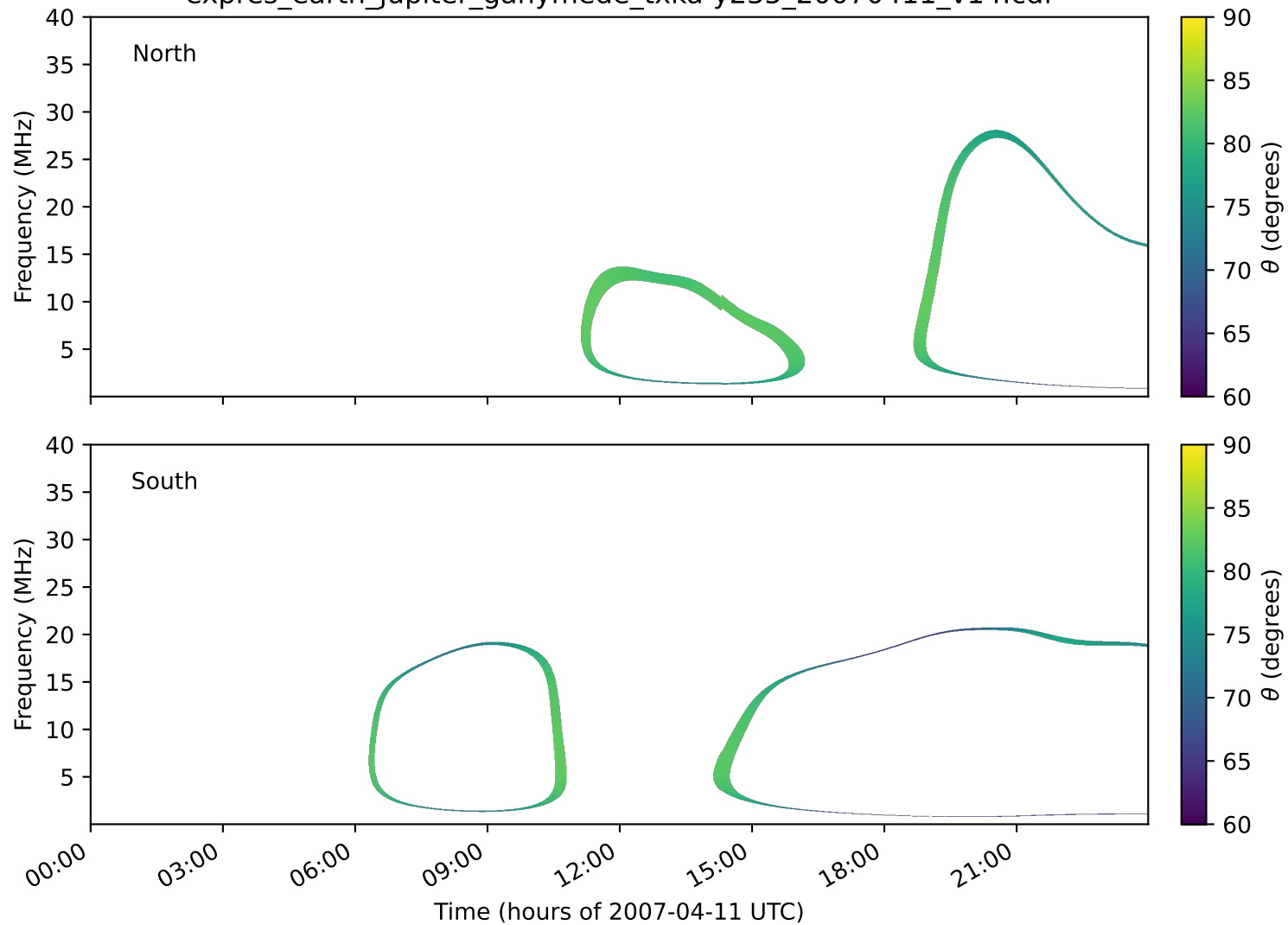
expres_earth_jupiter_ganymede_txka-y235_20070411_v14.cdf
