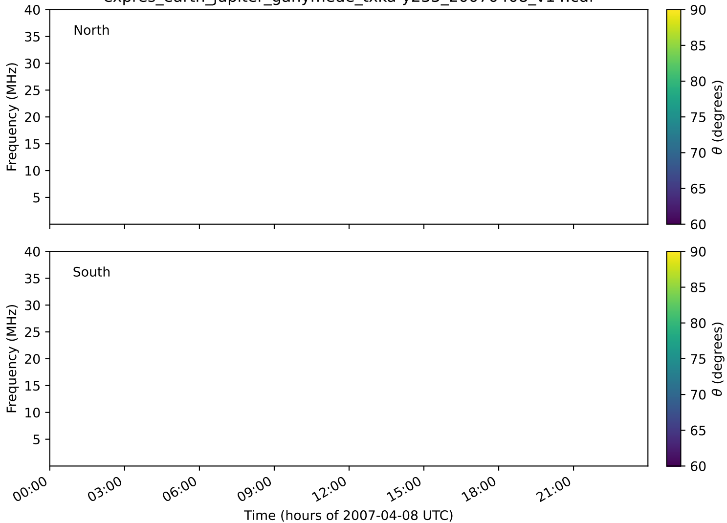
expres_earth_jupiter_ganymede_txka-y235_20070408_v14.cdf
