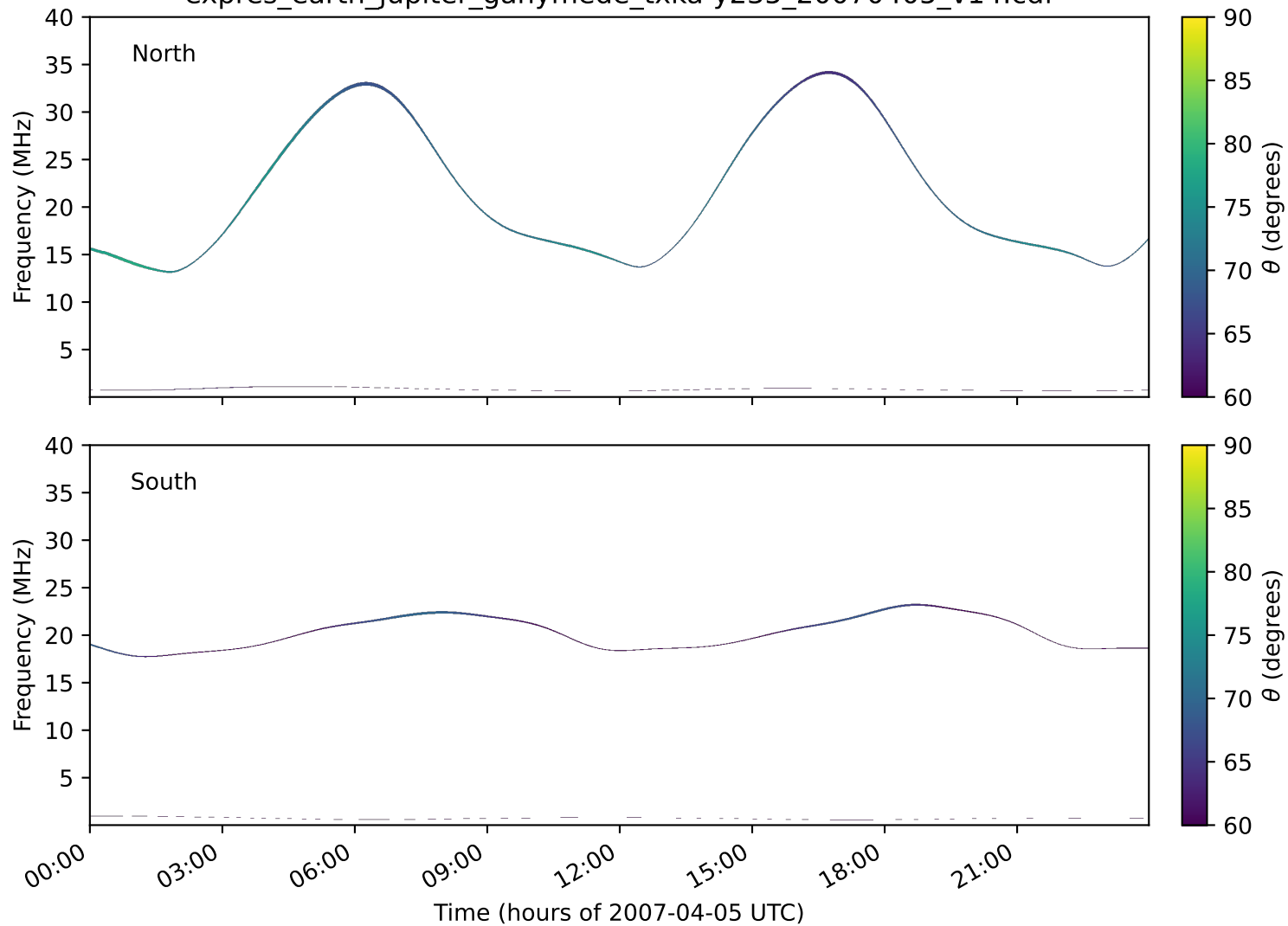
expres_earth_jupiter_ganymede_txka-y235_20070405_v14.cdf
