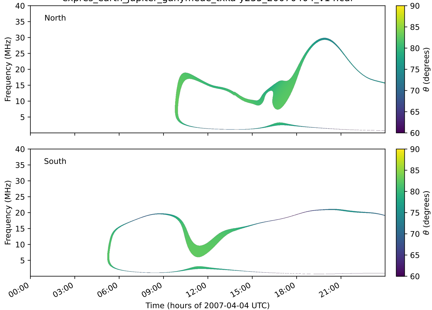
expres_earth_jupiter_ganymede_txka-y235_20070404_v14.cdf
