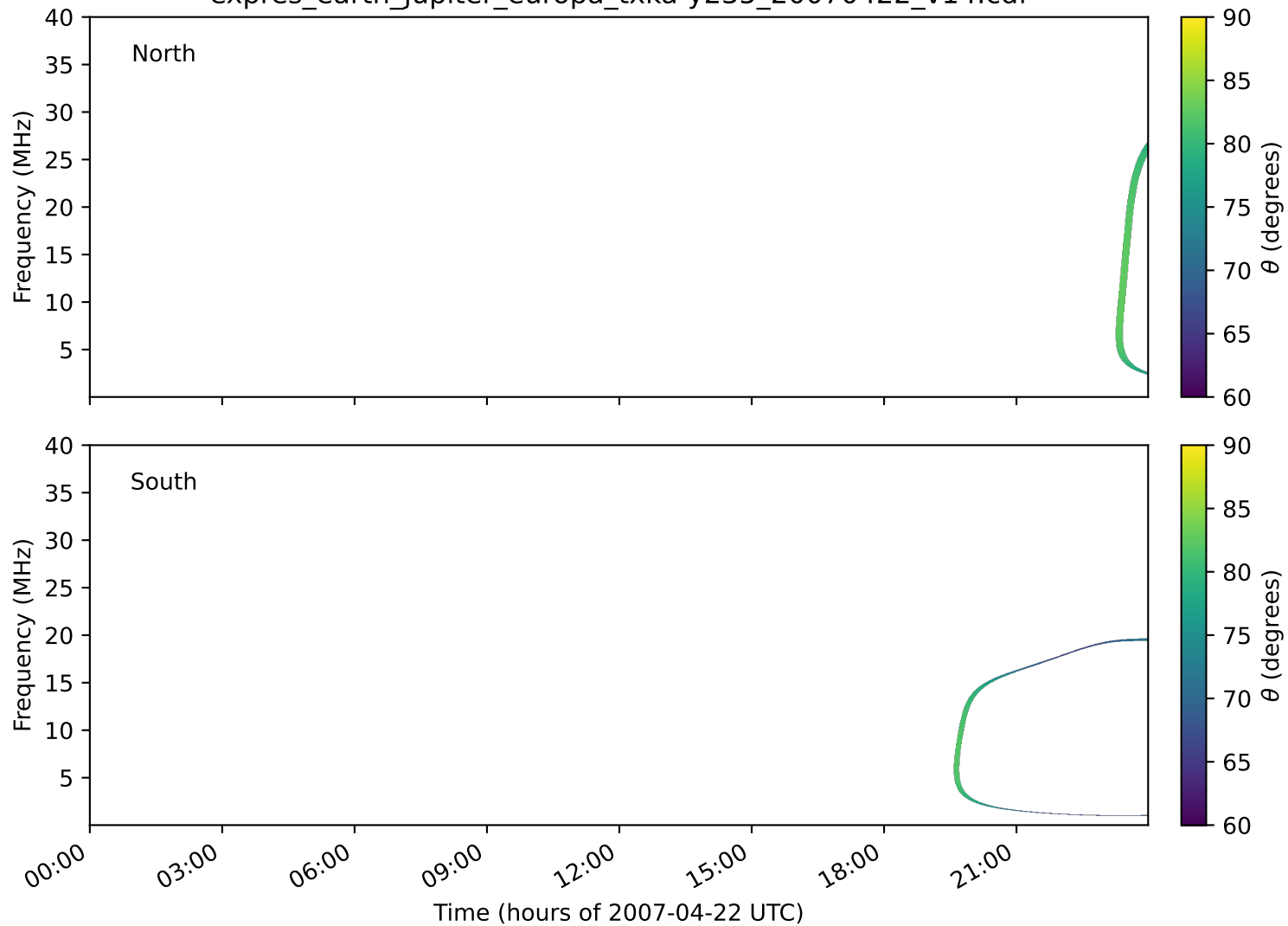
expres_earth_jupiter_europa_txka-y235_20070422_v14.cdf
