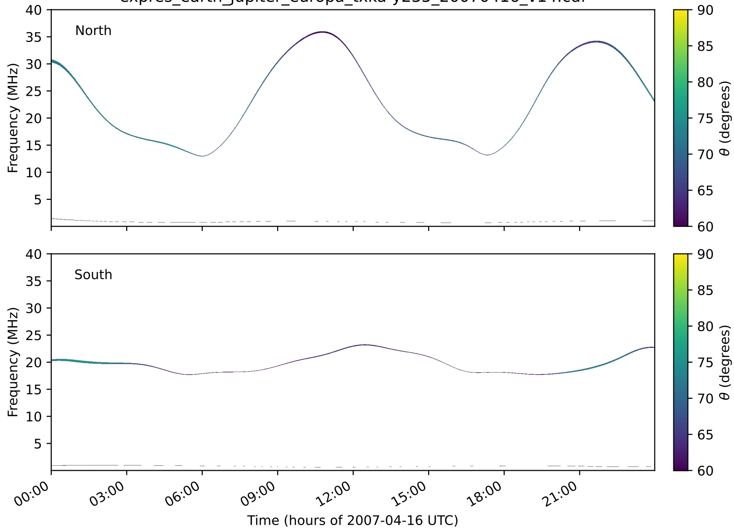
expres_earth_jupiter_europa_txka-y235_20070416_v14.cdf
