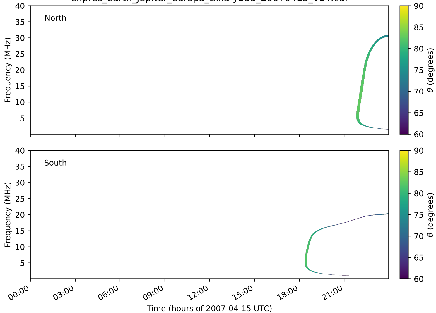
expres_earth_jupiter_europa_txka-y235_20070415_v14.cdf
