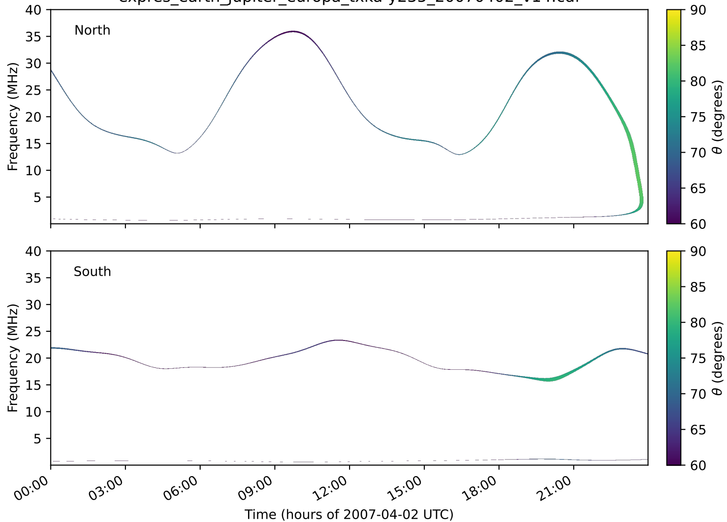
expres_earth_jupiter_europa_txka-y235_20070402_v14.cdf
