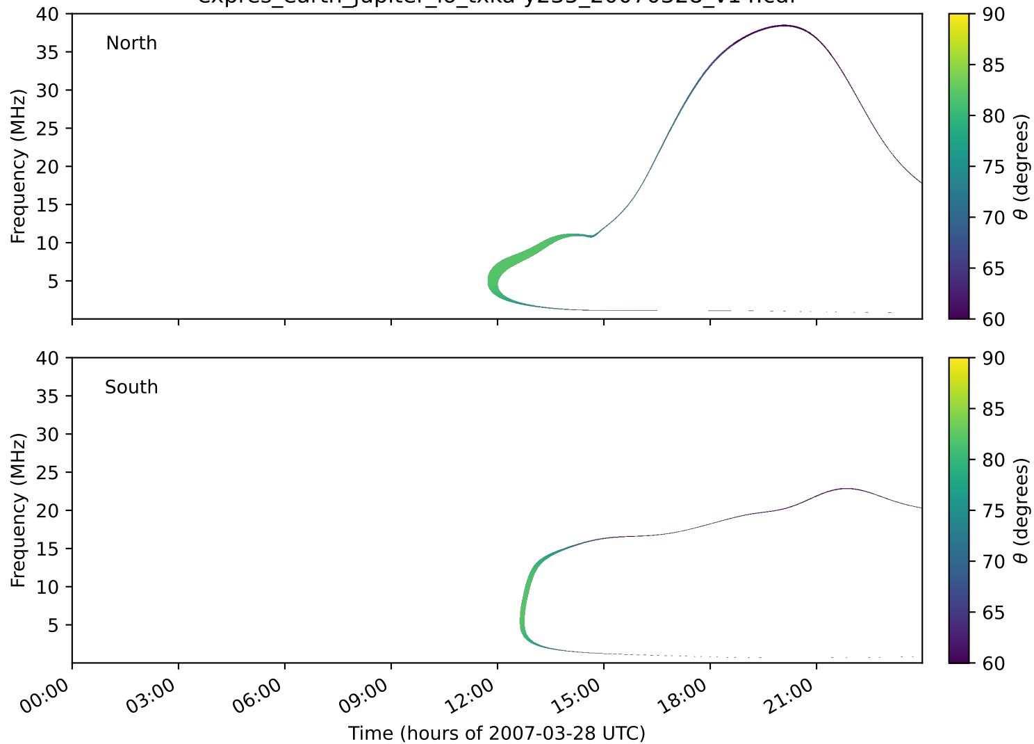
expres_earth_jupiter_io_txka-y235_20070328_v14.cdf
