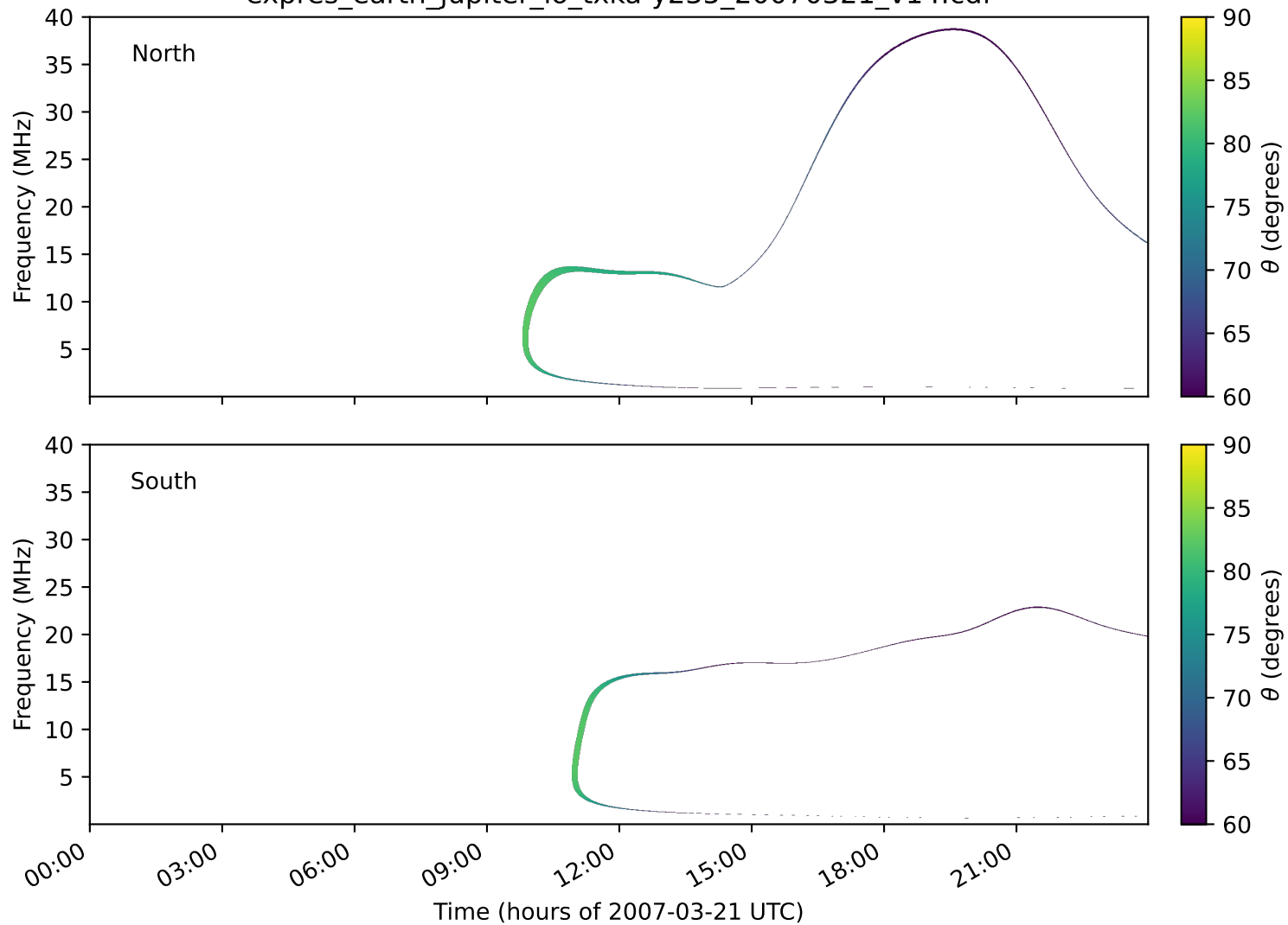
expres_earth_jupiter_io_txka-y235_20070321_v14.cdf
