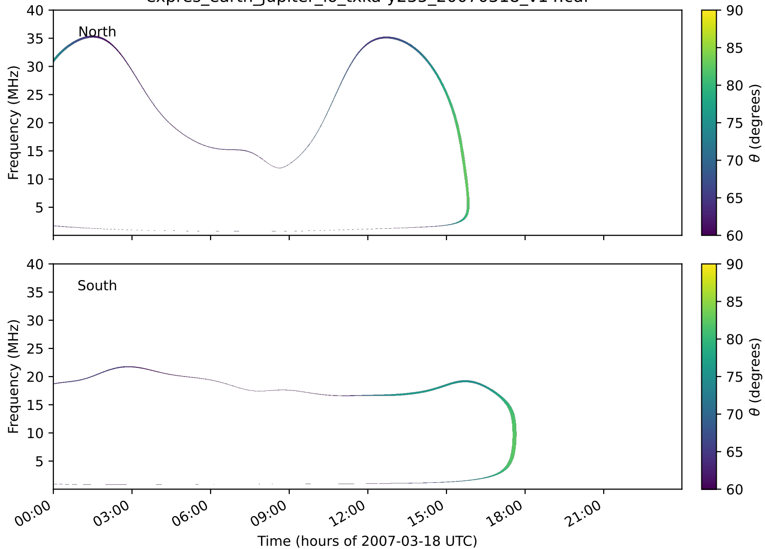
expres_earth_jupiter_io_txka-y235_20070318_v14.cdf
