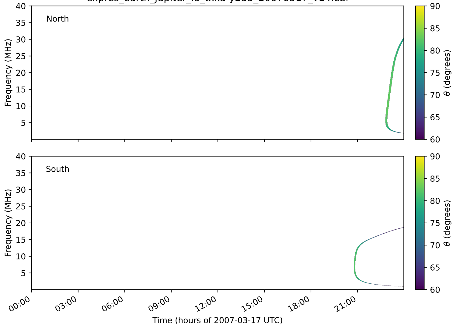
expres_earth_jupiter_io_txka-y235_20070317_v14.cdf
