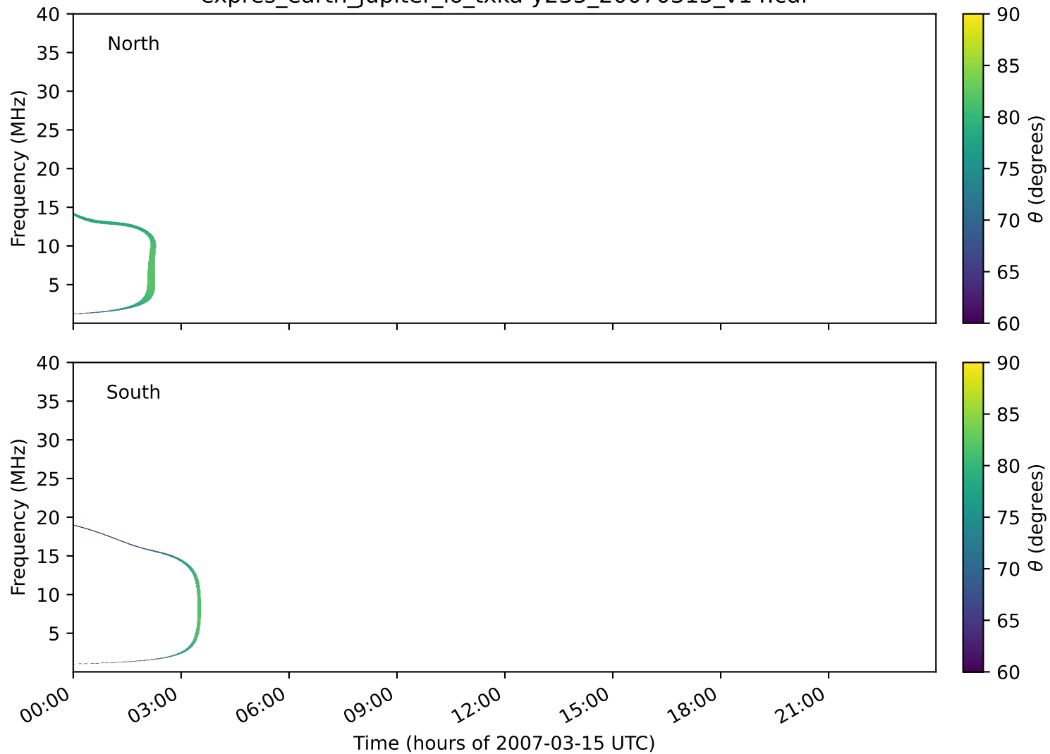
expres_earth_jupiter_io_txka-y235_20070315_v14.cdf
