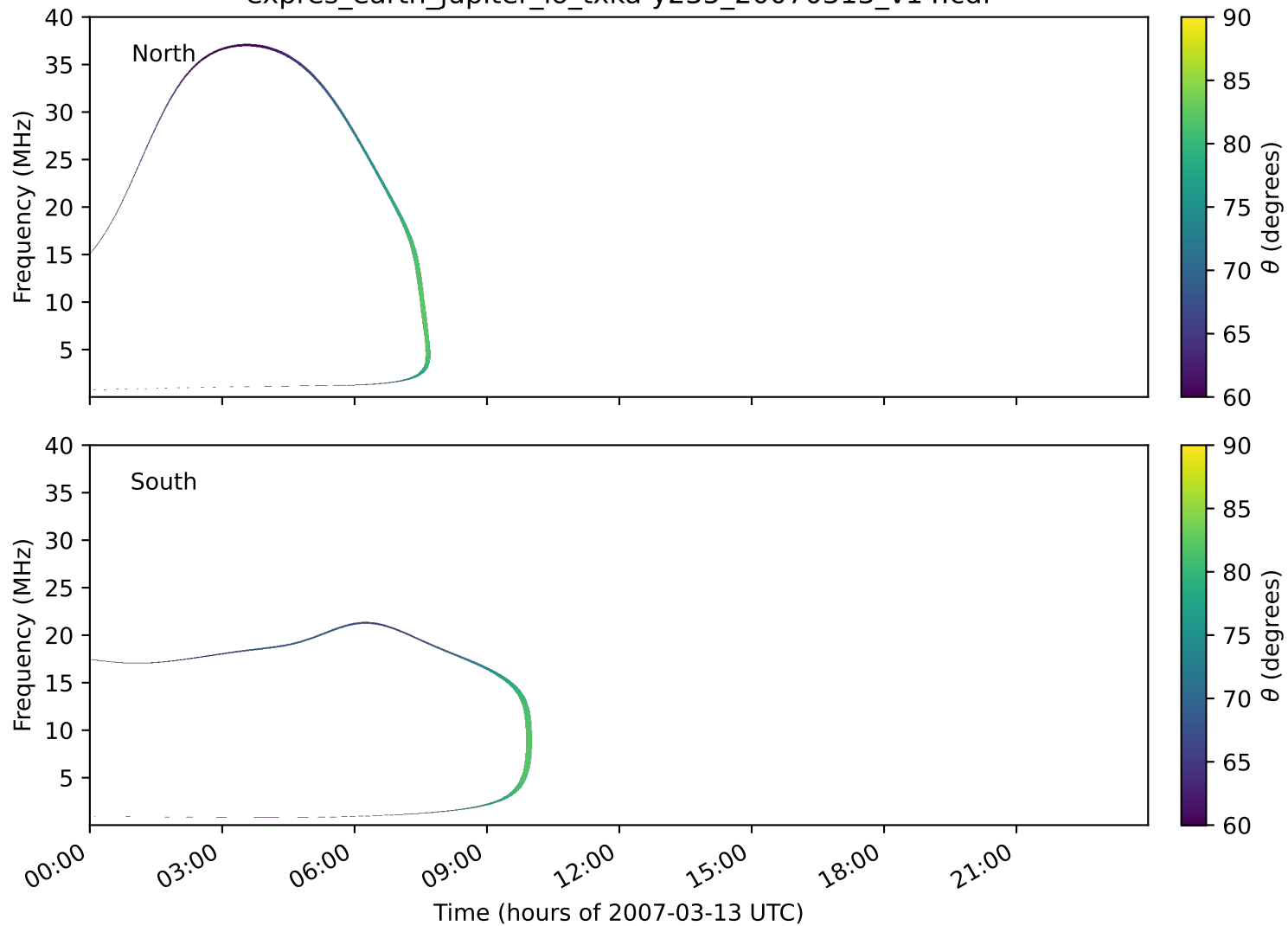
expres_earth_jupiter_io_txka-y235_20070313_v14.cdf
