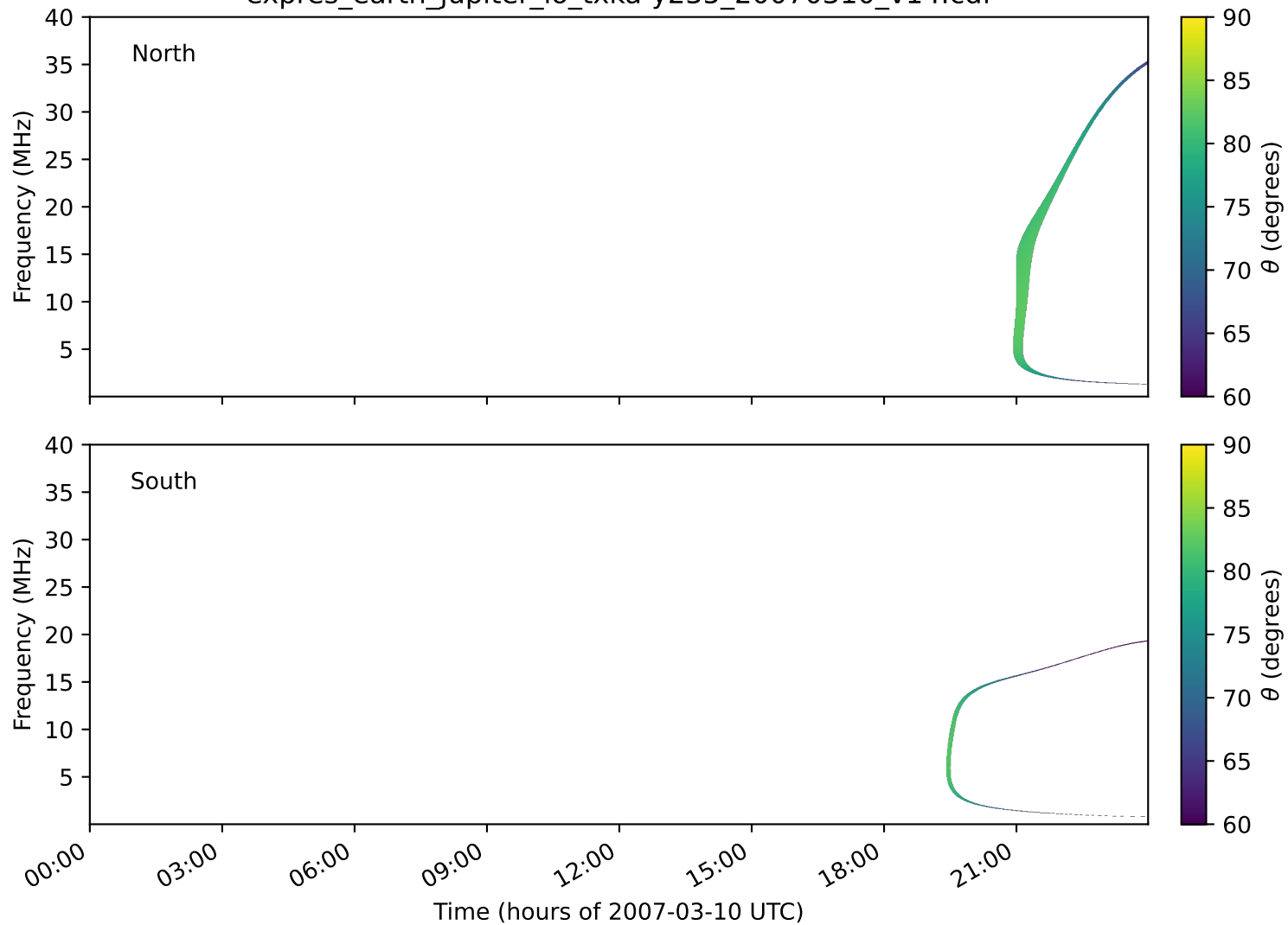
expres_earth_jupiter_io_txka-y235_20070310_v14.cdf
