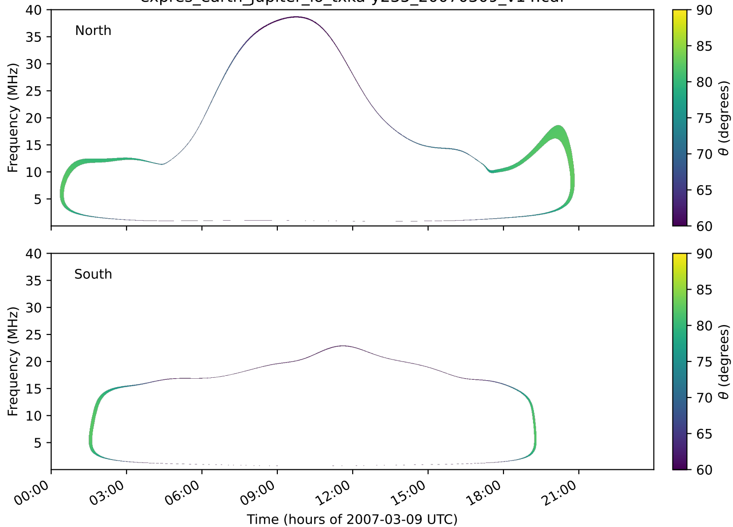
expres_earth_jupiter_io_txka-y235_20070309_v14.cdf
