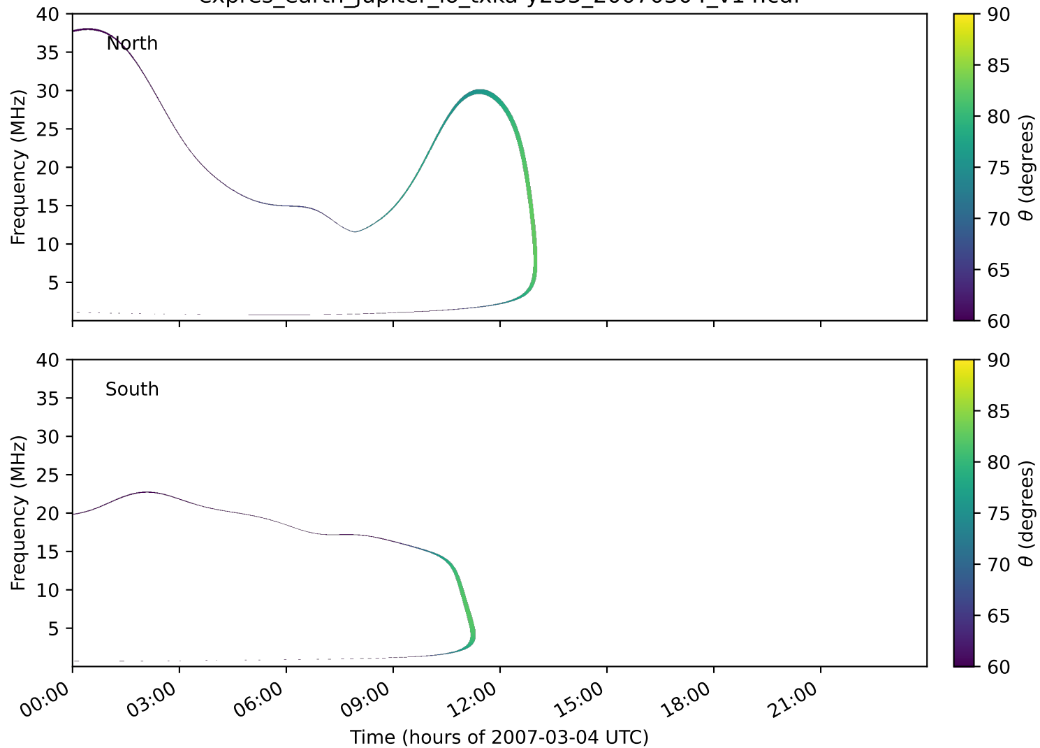
expres_earth_jupiter_io_txka-y235_20070304_v14.cdf
