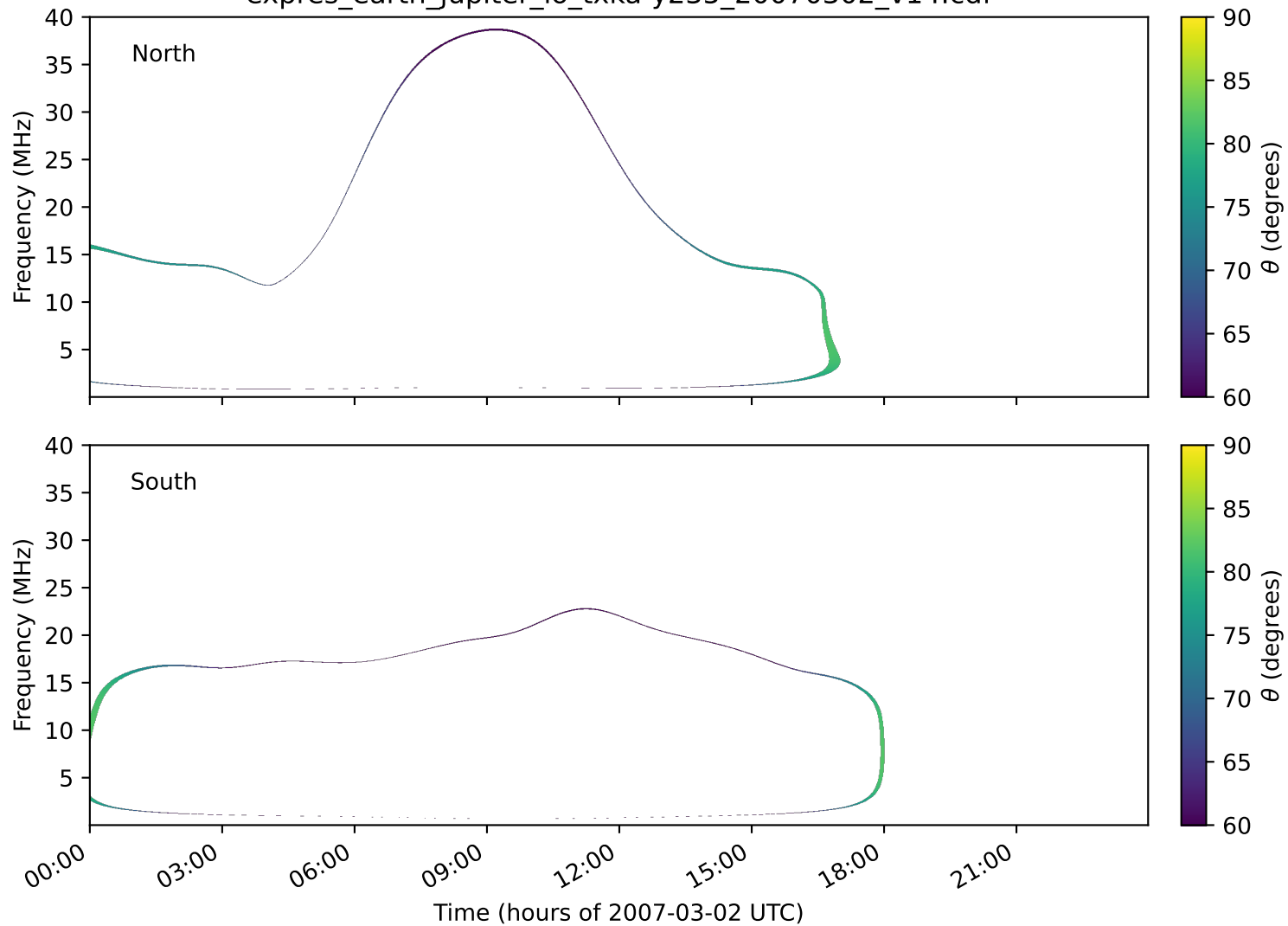
expres_earth_jupiter_io_txka-y235_20070302_v14.cdf
