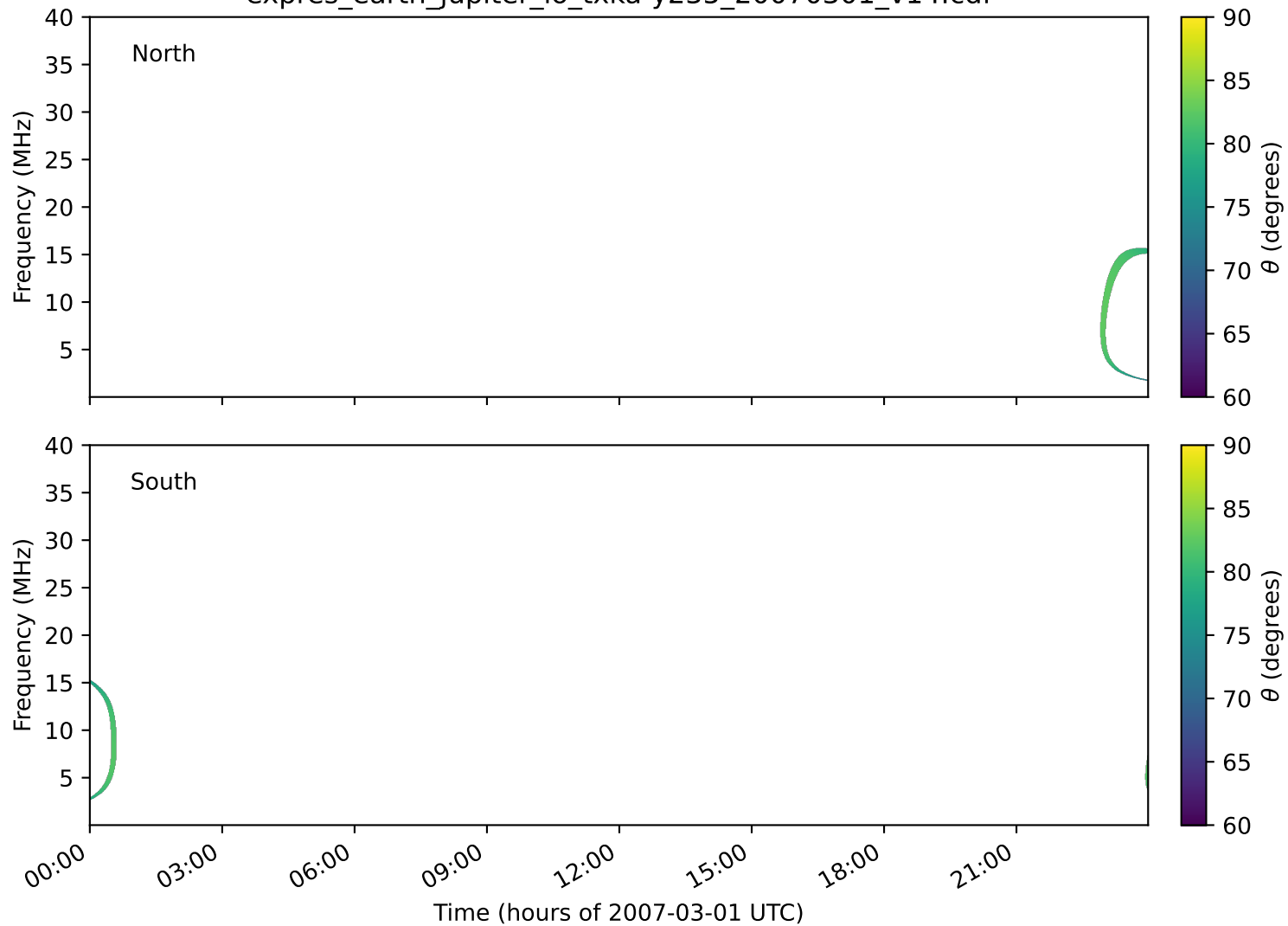
expres_earth_jupiter_io_txka-y235_20070301_v14.cdf
