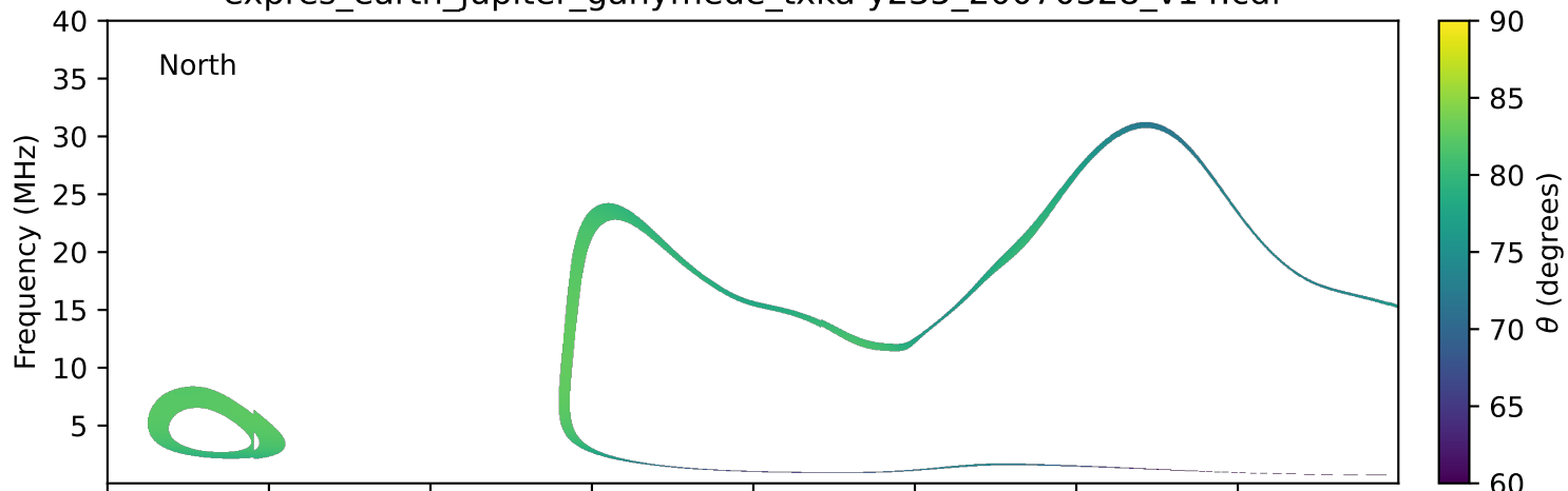
expres_earth_jupiter_ganymede_txka-y235_20070328_v14.cdf
