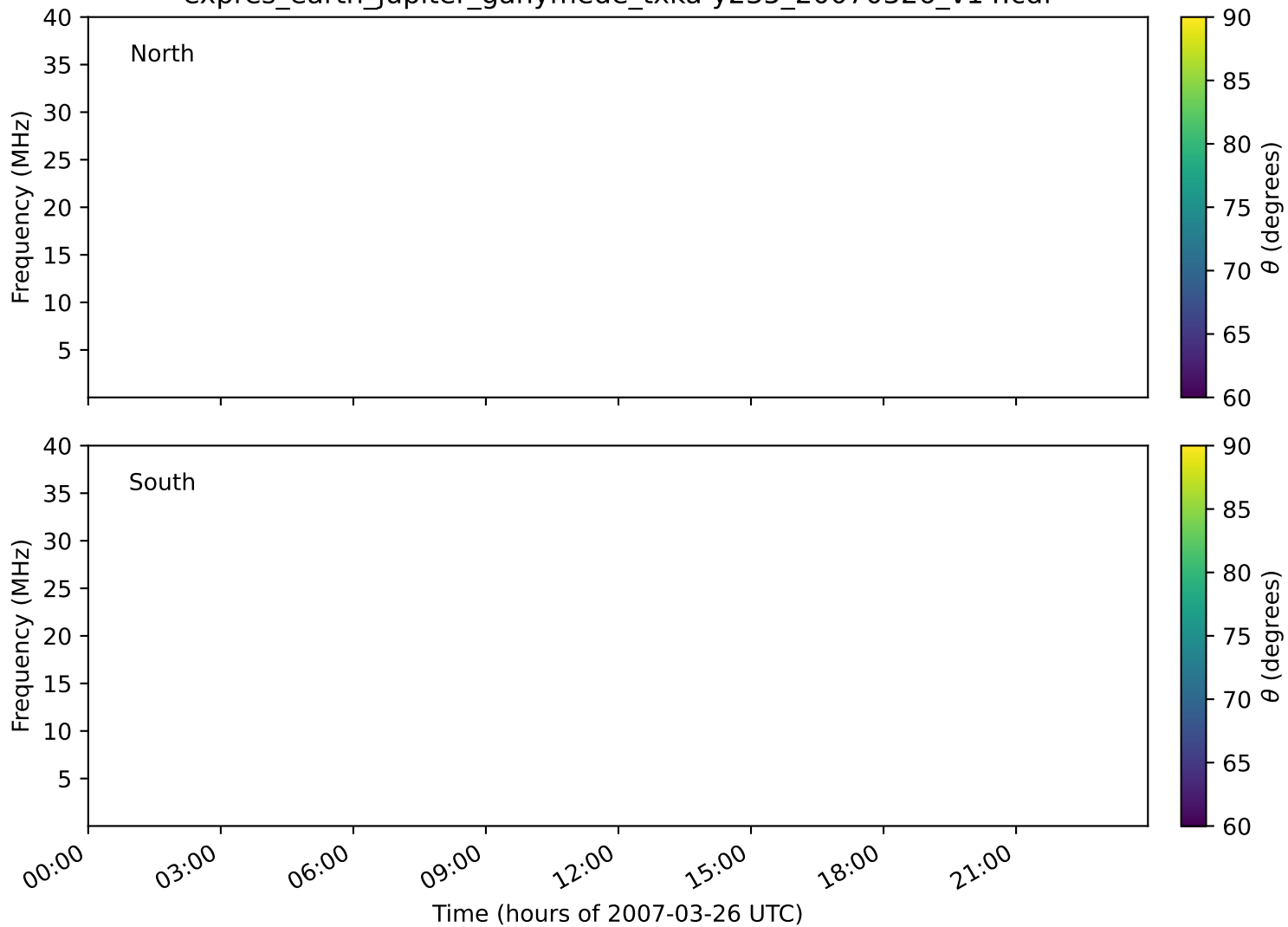
expres_earth_jupiter_ganymede_txka-y235_20070326_v14.cdf
