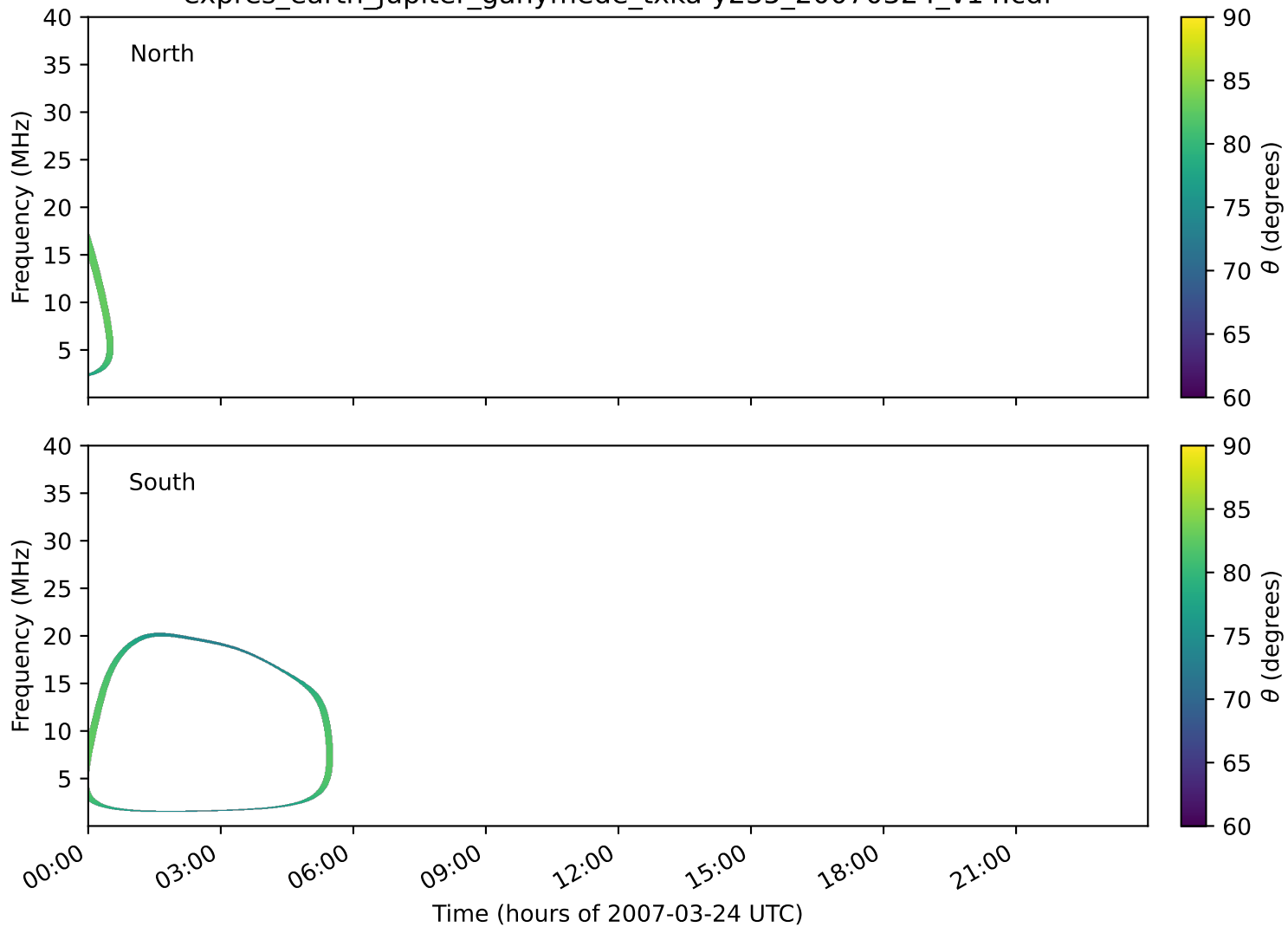
expres_earth_jupiter_ganymede_txka-y235_20070324_v14.cdf
