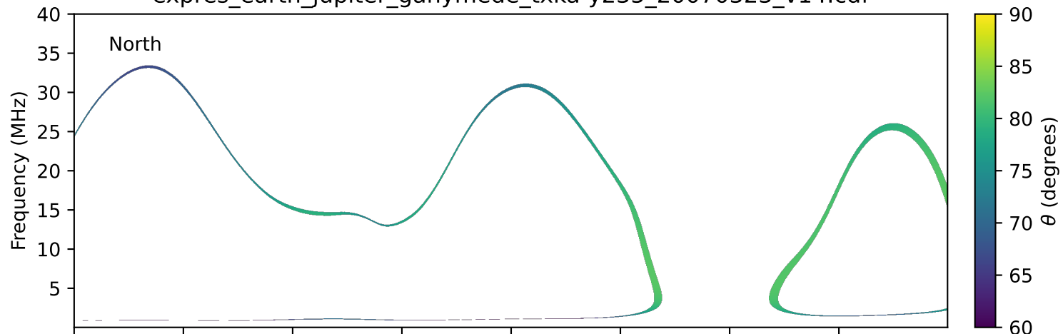
expres_earth_jupiter_ganymede_txka-y235_20070323_v14.cdf
