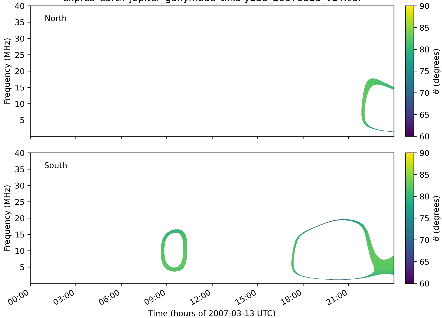
expres_earth_jupiter_ganymede_txka-y235_20070313_v14.cdf
