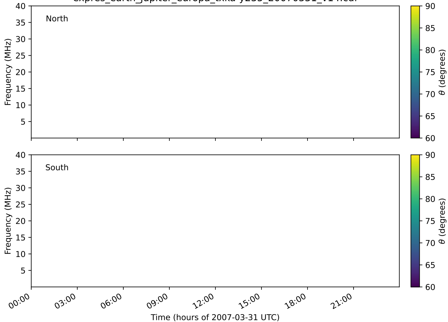
expres_earth_jupiter_europa_txka-y235_20070331_v14.cdf
