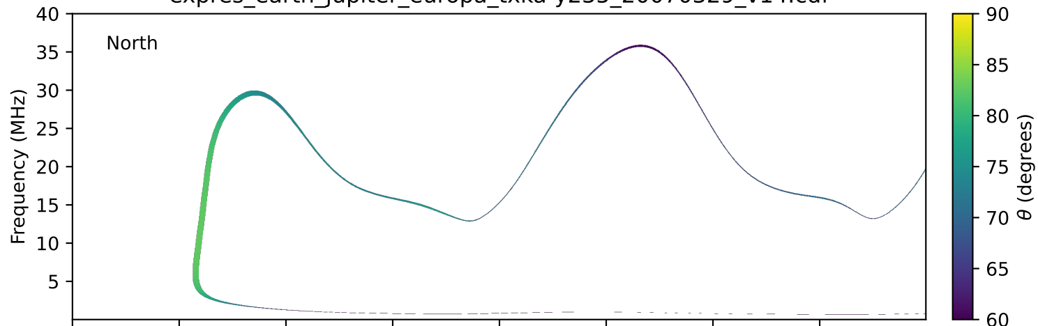
expres_earth_jupiter_europa_txka-y235_20070329_v14.cdf
