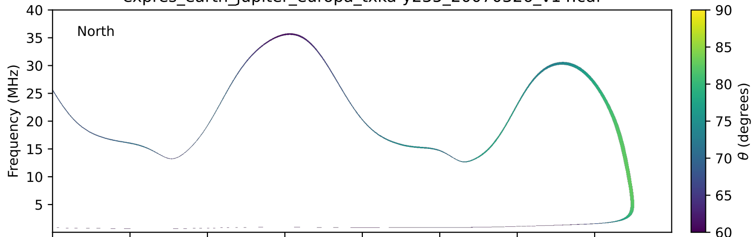
expres_earth_jupiter_europa_txka-y235_20070326_v14.cdf
