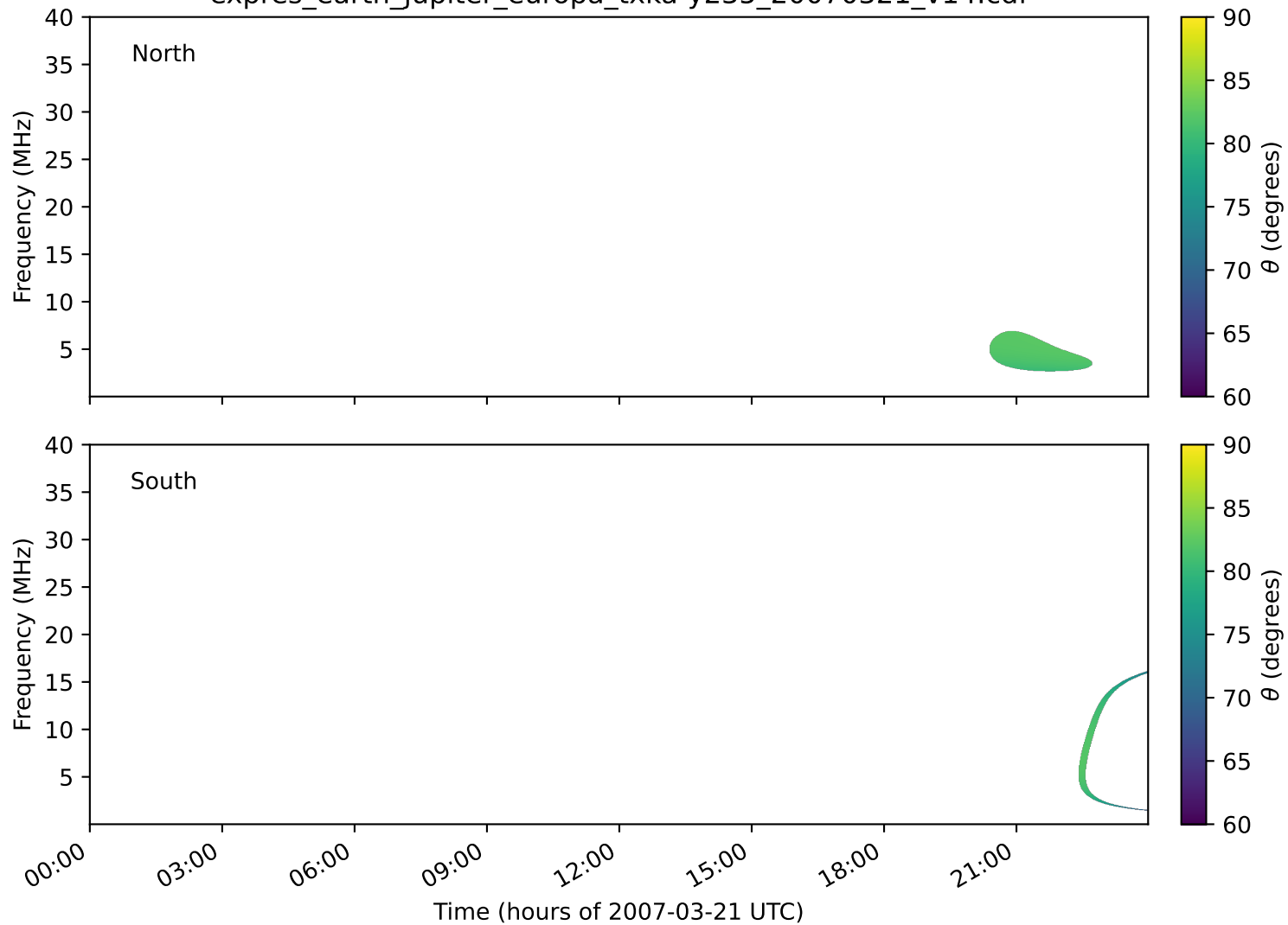
expres_earth_jupiter_europa_txka-y235_20070321_v14.cdf
